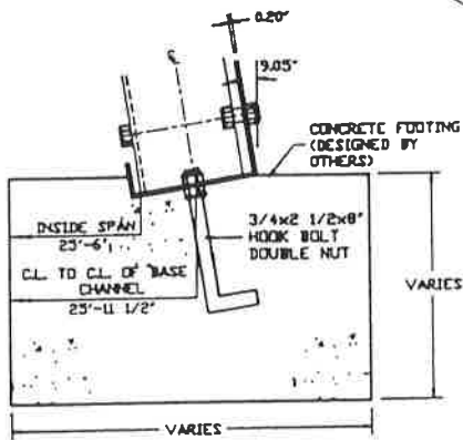
DETAIL #1 - BASE CHANNEL IN CONCRETE FOOTING
