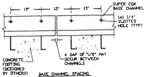
BASE CHANNEL SPACING
