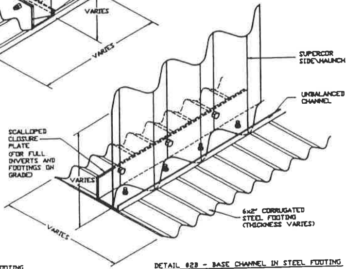
DETAIL #2B - BASE CHANNEL IN STEEL FOOTING
