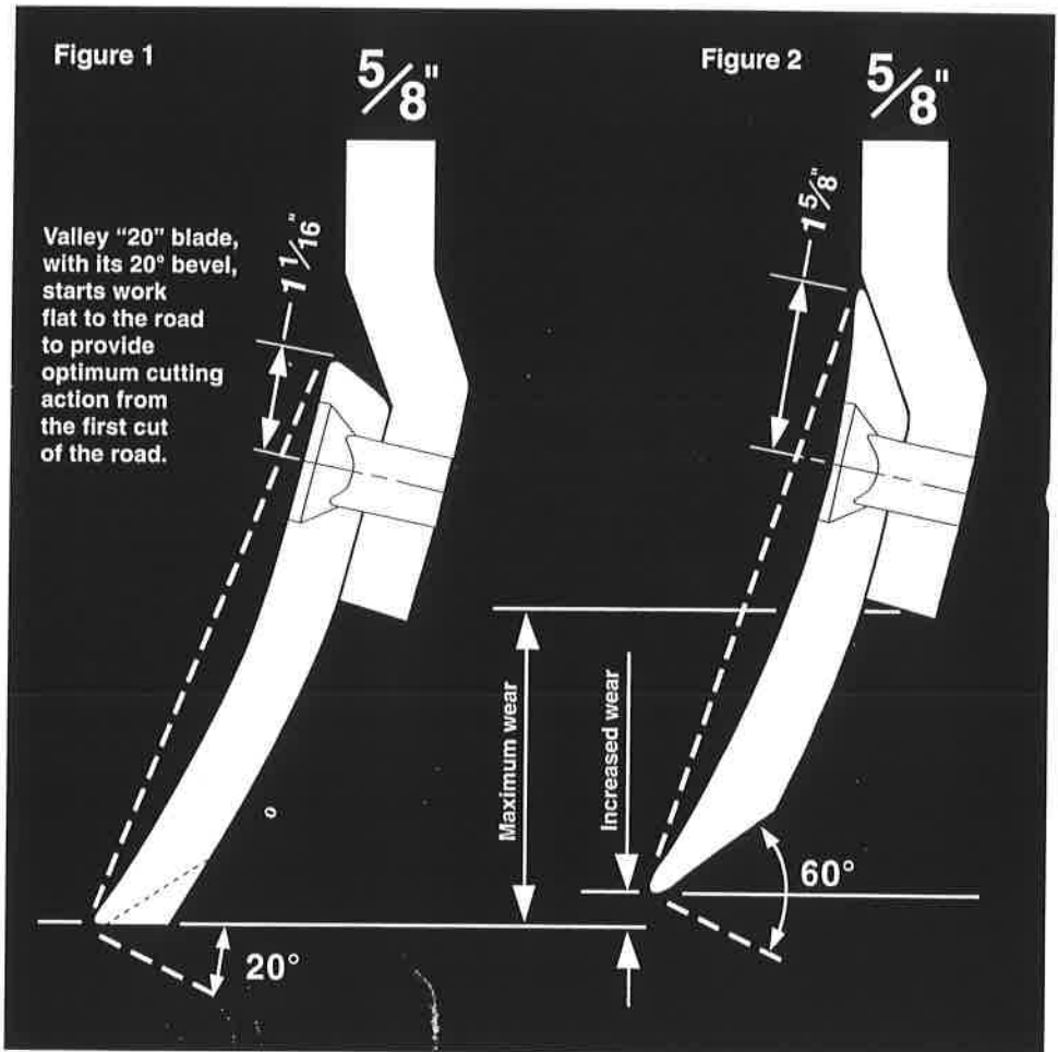
Figure 1: Valley "20" Grader Blade
