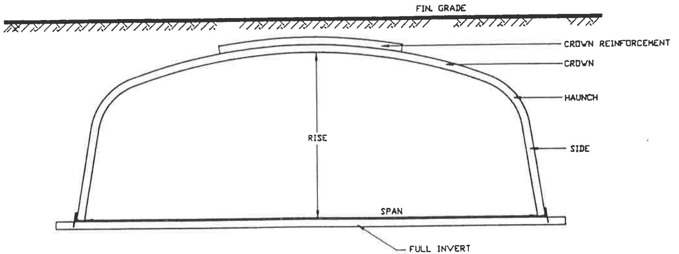
Typical Detail - Full Invert
