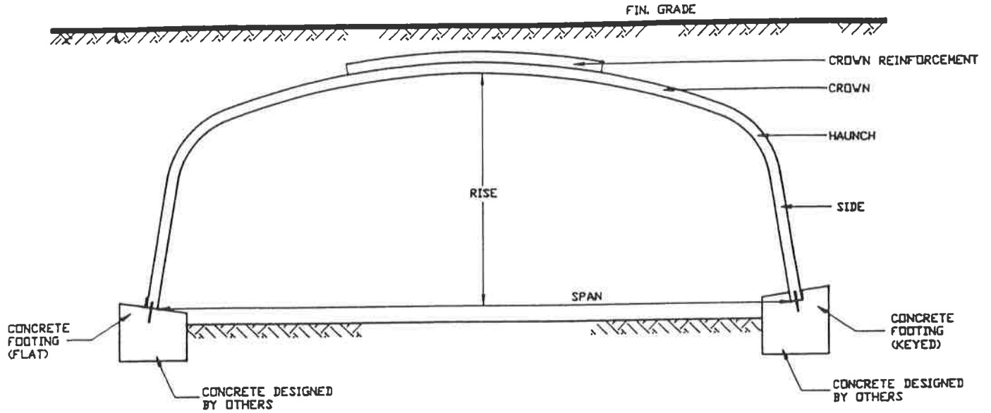
Typical Detail - Super·Cor™ on Concrete Footing
